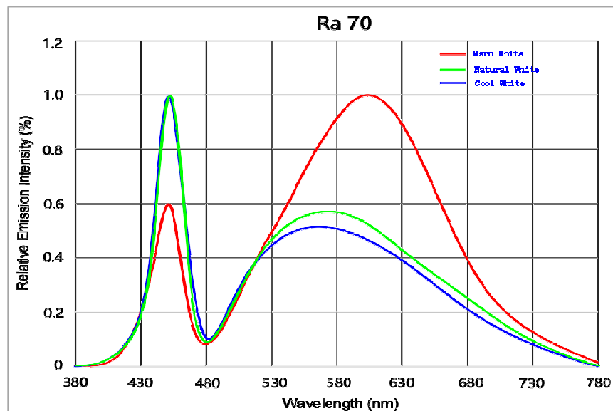
Fig.1-Spectrum Distribution
