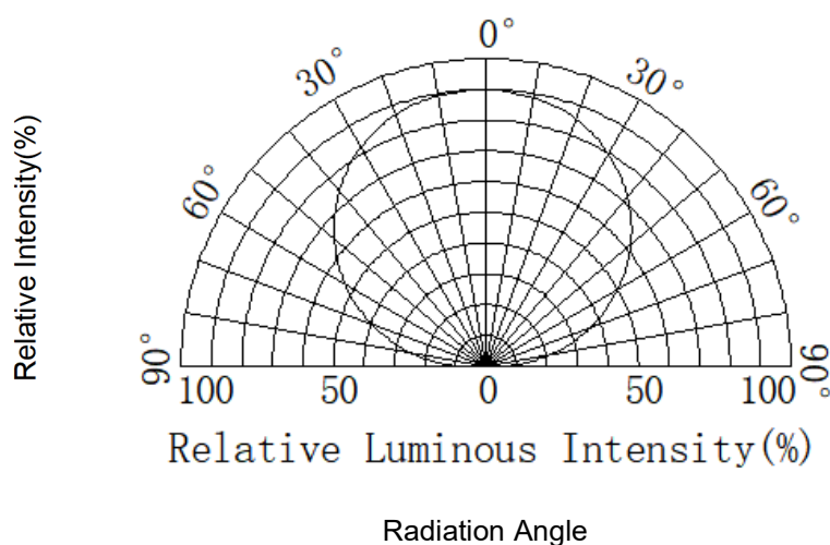
Fig.6- Directivity
